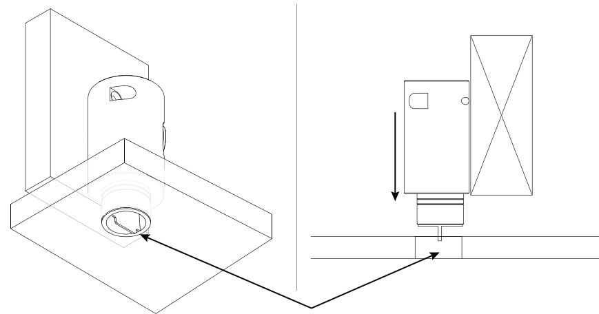
Drill a 1 1/8" (29 mm) hole for the Micro J-box. Remove red plug after mud dries.
